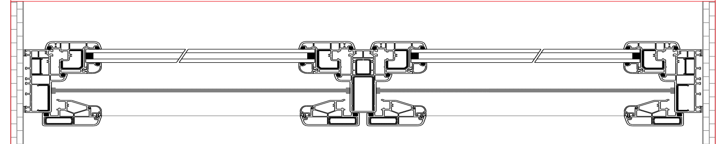
Cross Section
